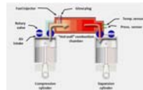
Basic elements of the Zajac engine.
